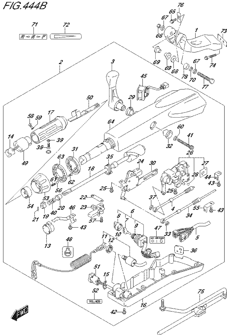
FIG.444B (2-H-9) TILLER HANDLE (DF70ATH E40)
